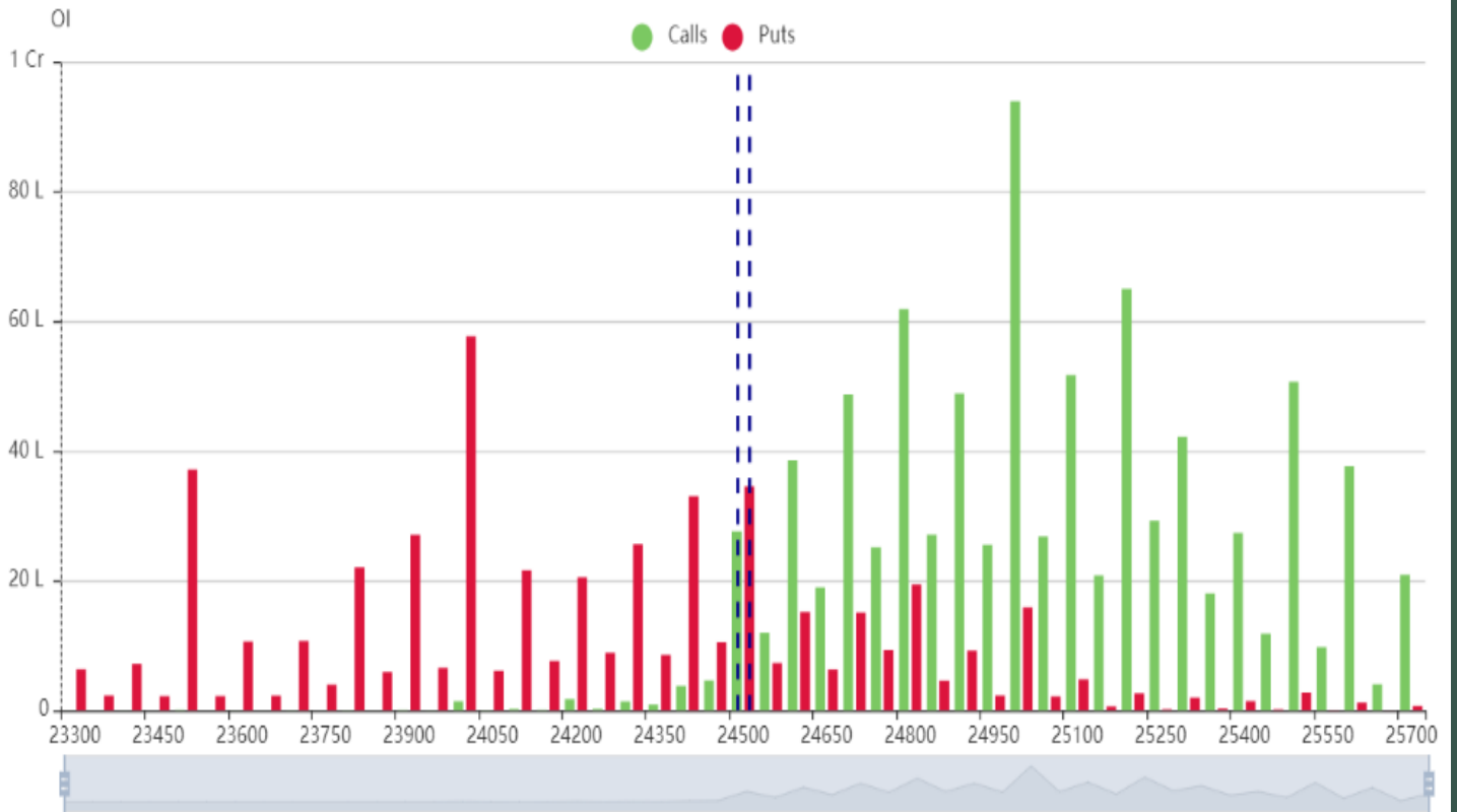
NIFTY-24OCT24 Open Interest
