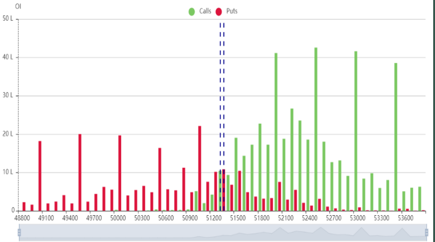
BANKNIFTY-23OCT24 Open Interest
